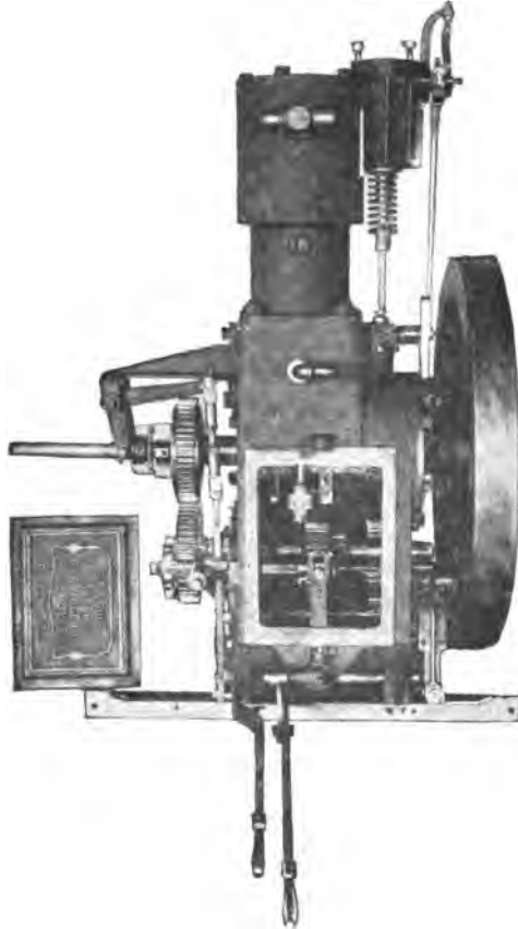
FIG. 401.—Single Cylinder Motor of the St. Louis Gasoline Motor Carriage, showing control levers and the variable speed gear contained within the case below the crank.
